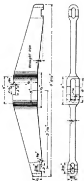
Figs. 1652-1653. Equalizer for Eight-Wheel (1-4-0) Locomotive. C., C., C. & St. L.
